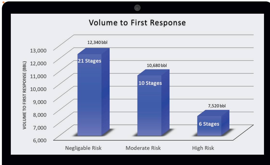
Above: Volume to first response in offset well measured by fiber optics compared to fracture risk as identified by Drill2Frac.
